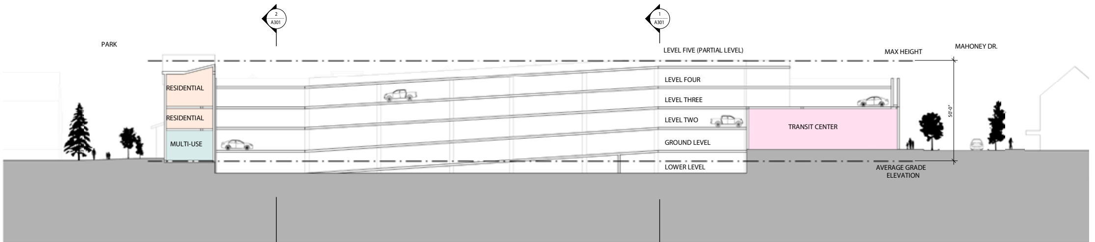
3 SITE SECTION - EAST / WEST A301 1" = 20'-0"
