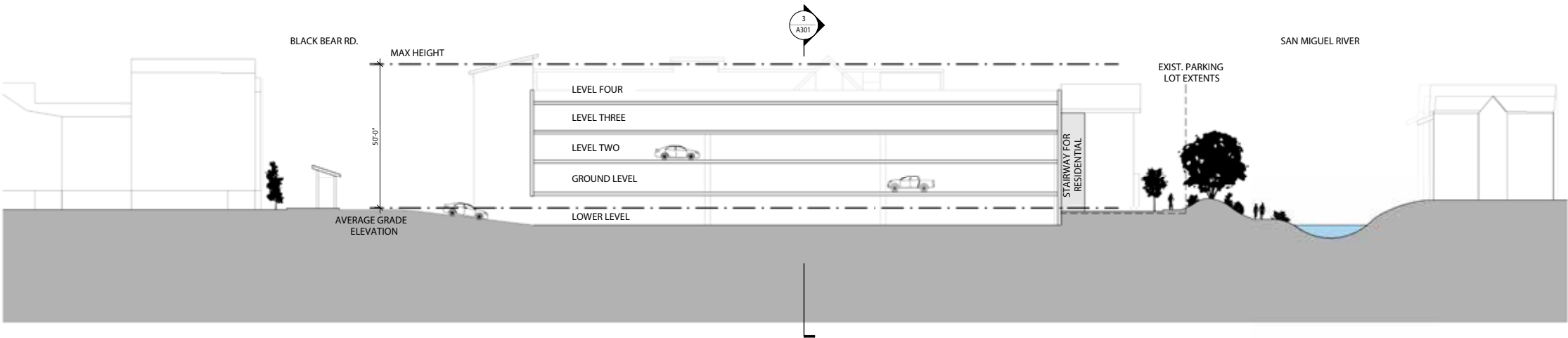
2 SITE SECTION - NORTH / SOUTH - VIEW 2 A301 1" = 20'-0"
