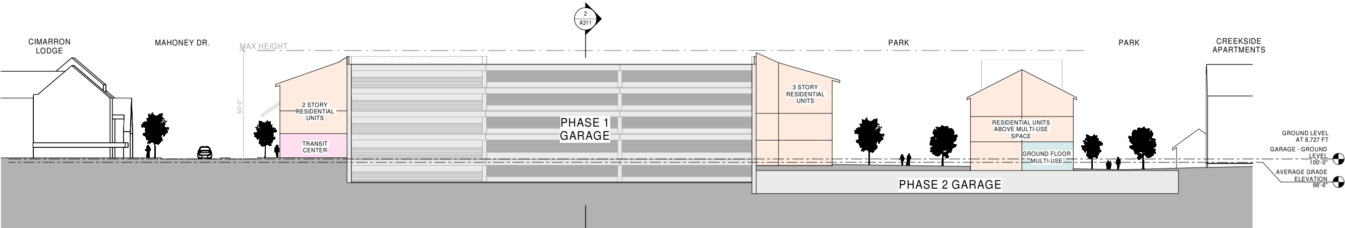
3 SITE SECTION - EAST / WEST - VIEW 2 A311 1" = 20'-0"
