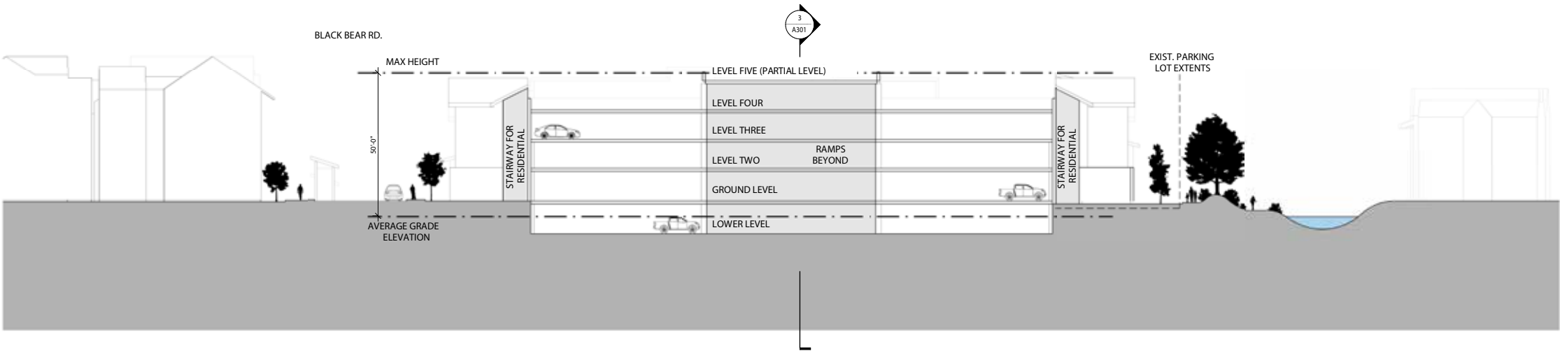
1 SITE SECTION - NORTH / SOUTH - VIEW 1 A301 1" = 20'-0"
