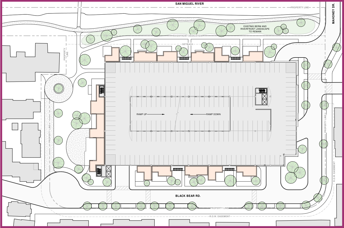
Alternate 1 - Upper Levels
