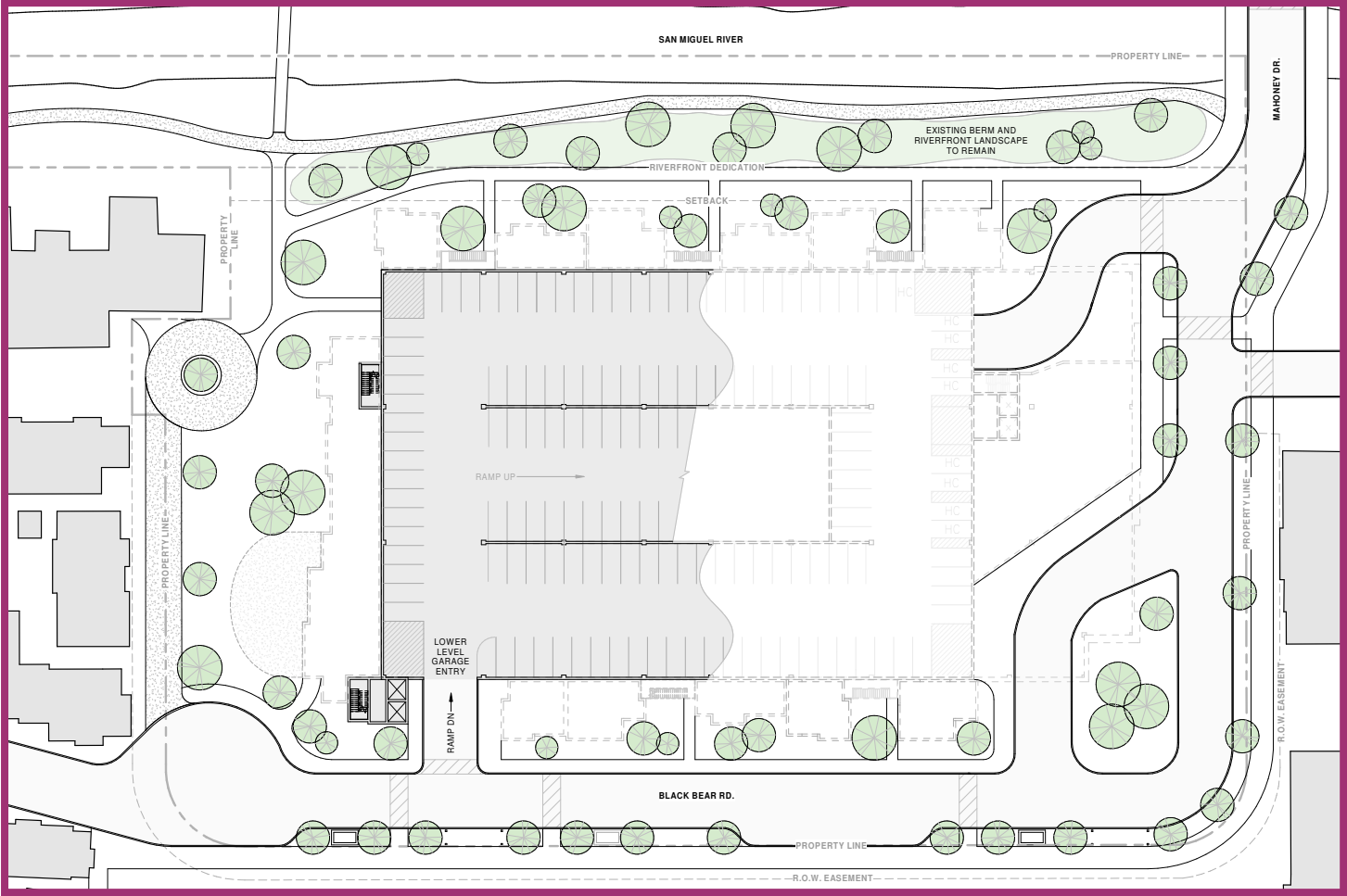
Alternate 1 - Basement Level
