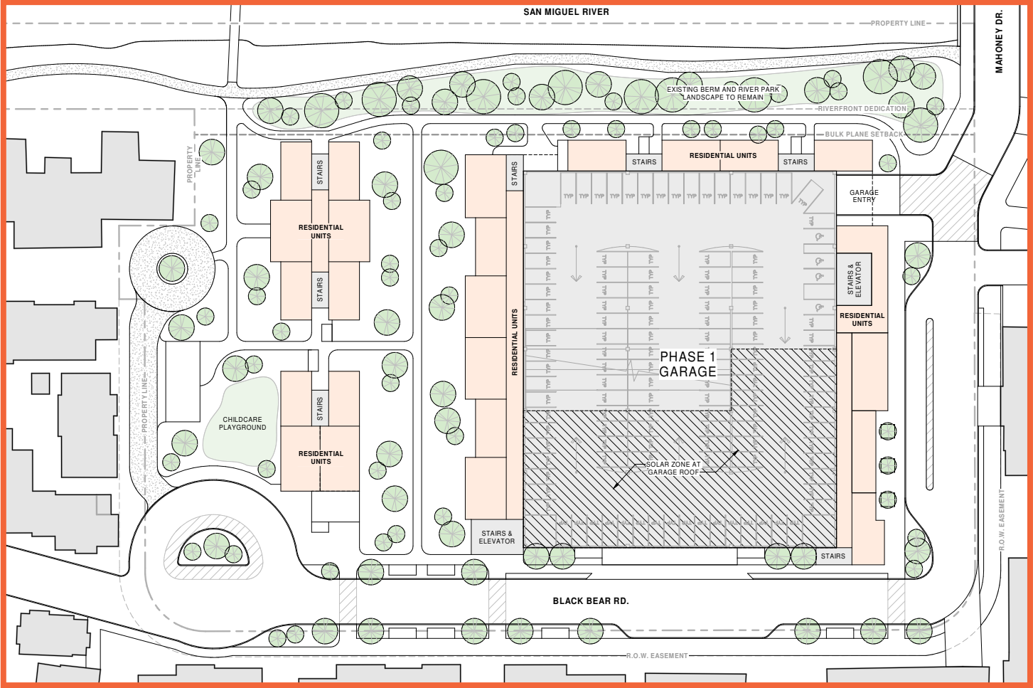
Alternate 2 - Upper Levels
