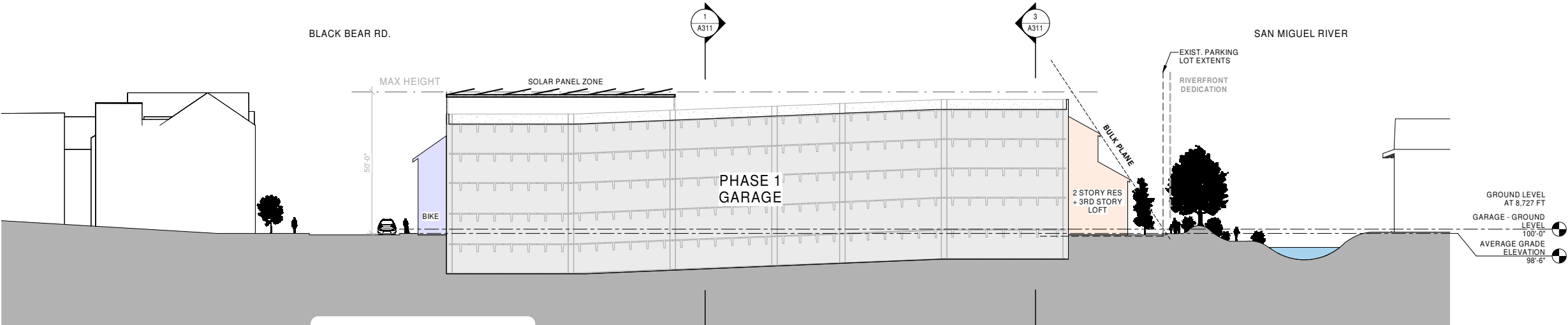
2 SITE SECTION - NORTH / SOUTH A311 1" = 20'-0"
