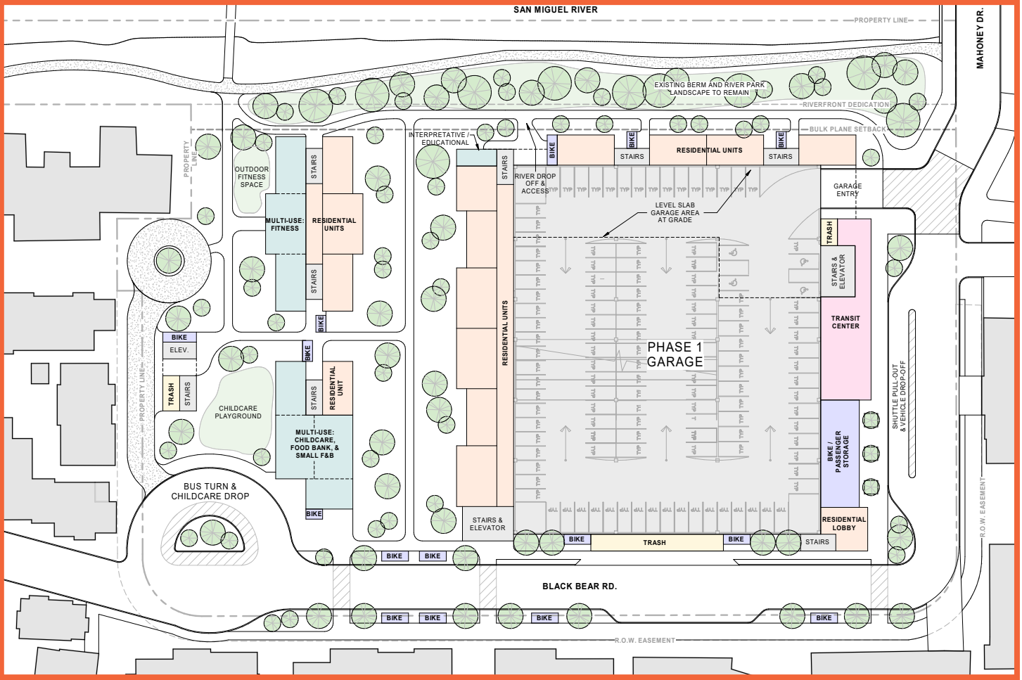
Alternate 2 - Ground Level
