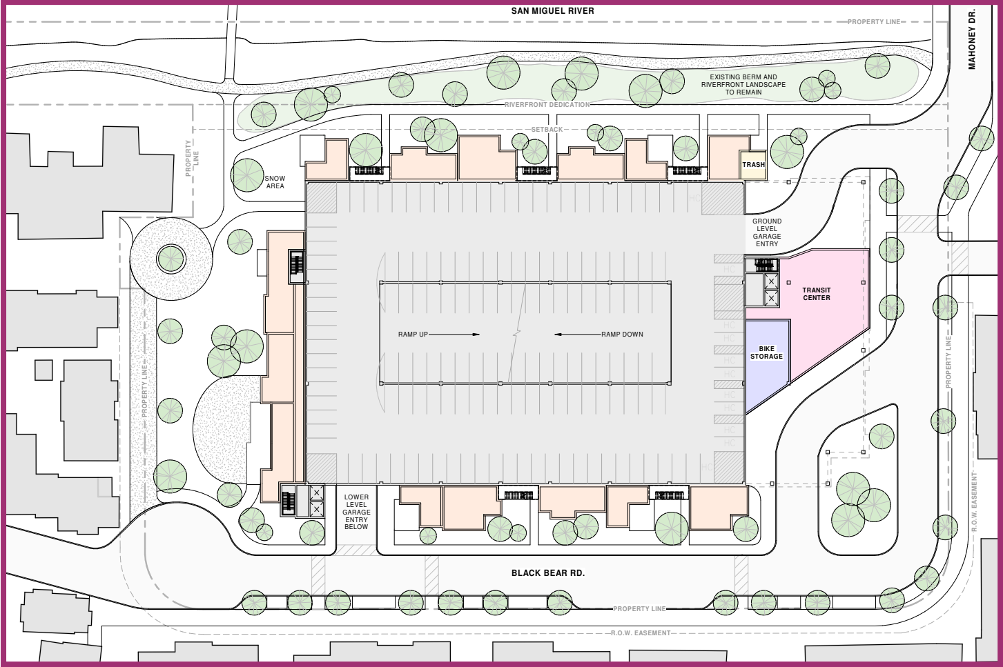
Alternate 1 - Ground Level
